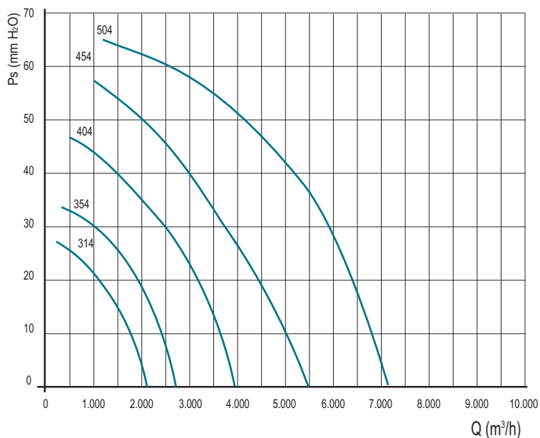
4 poli/4 poles (1500 rpm) - trifase/three-phase
