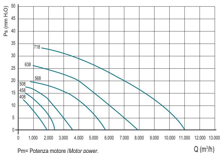
8 poli/8 poles (750 rpm) - trifase/three-phase
