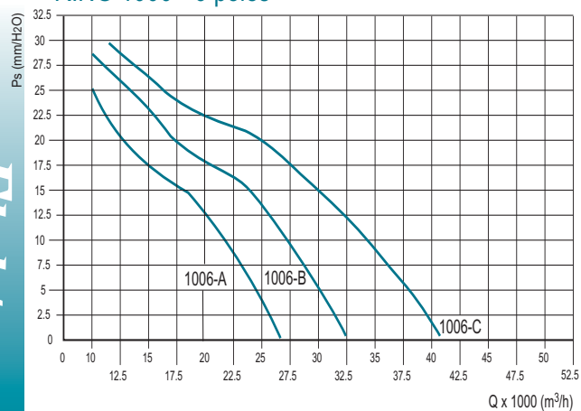
RING 1000 - 6 poles
