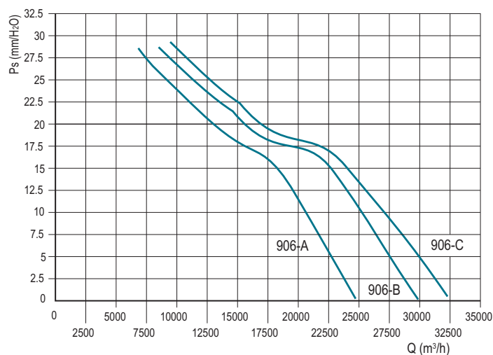
RING 900 - 6 poles
