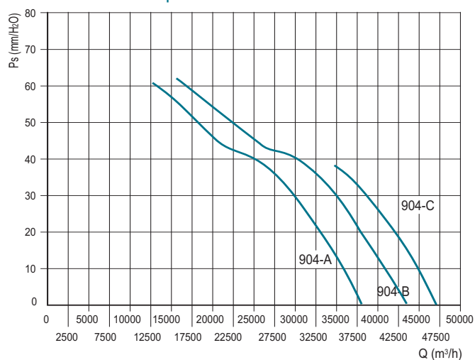
RING 900 - 4 poles
