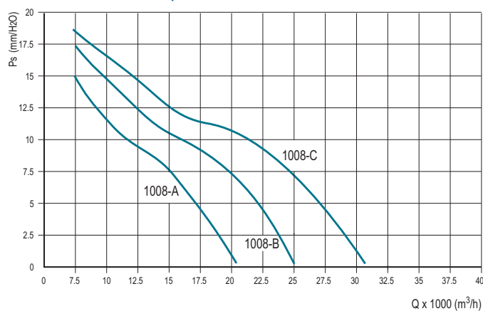
RING 1000 - 8 poles
