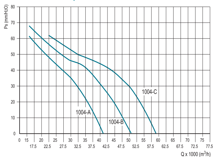
RING 1000 - 4 poles
