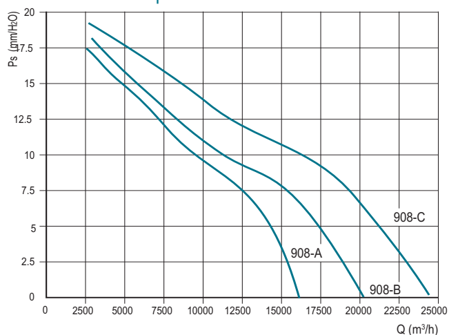
RING 900 - 8 poles
