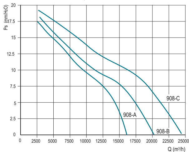
DUCT-M 900 - 8 poles
