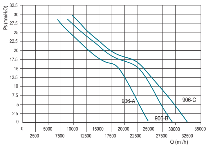
DUCT-M 900 - 6 poles
