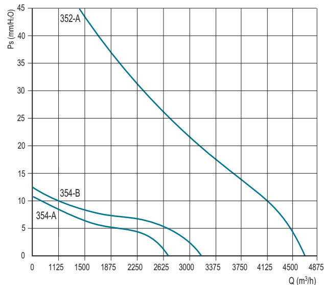
DUCT-M 350
