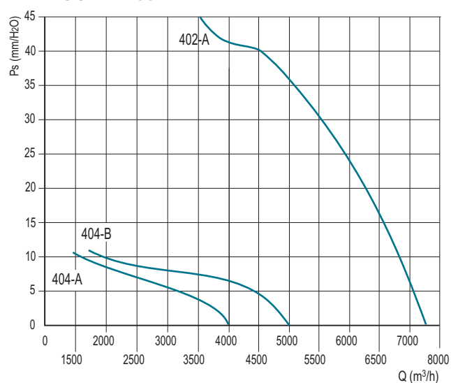
DUCT-M 400
