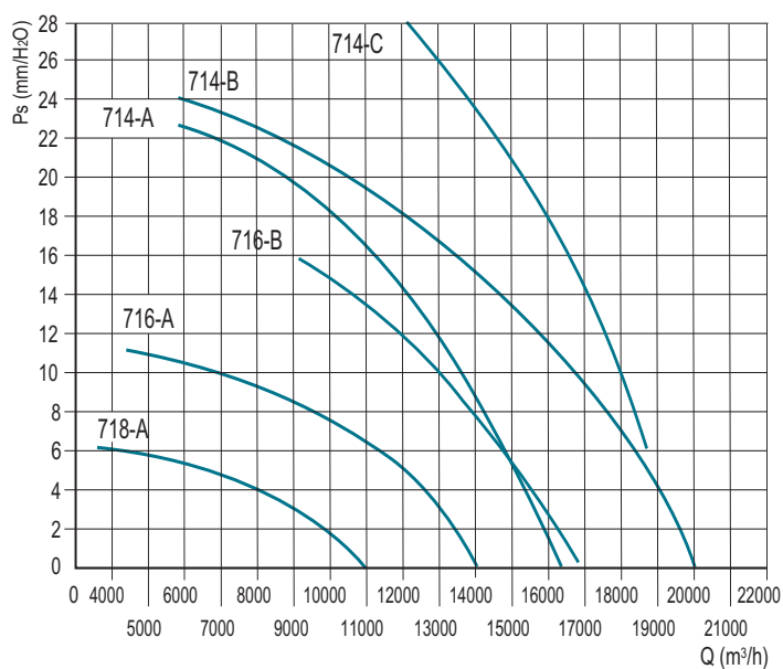
DUCT-M 800 - 6 poles
