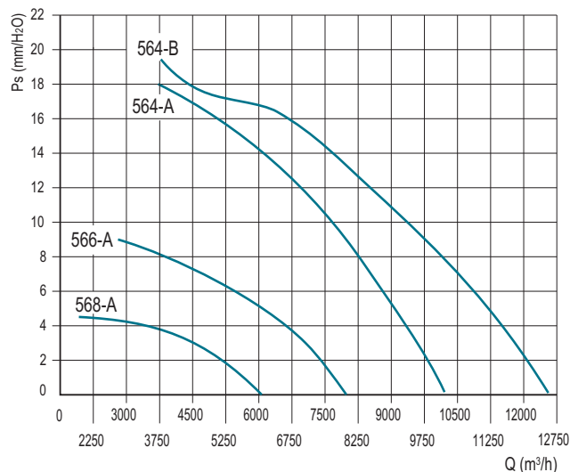
DUCT-M 560
