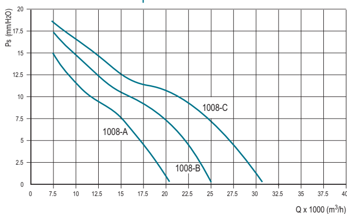
DUCT-M 1000 - 8 poles
