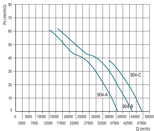
DUCT-M 900 - 4 poles
