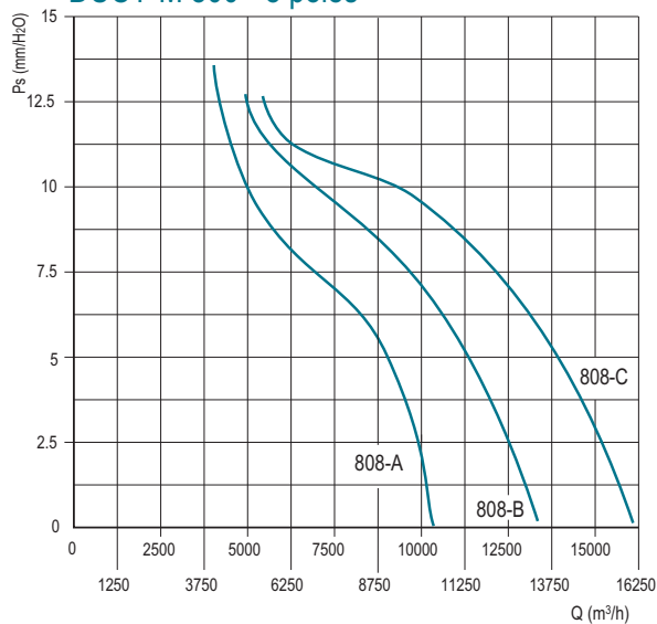
DUCT-M 800 - 8 poles
