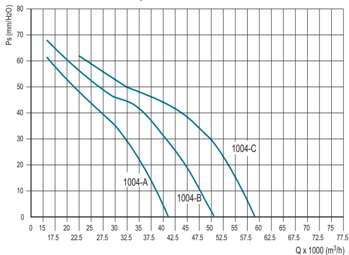
DUCT-M 1000 - 4 poles
