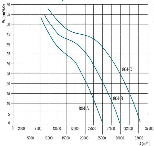
DUCT-M 800 - 8 poles
