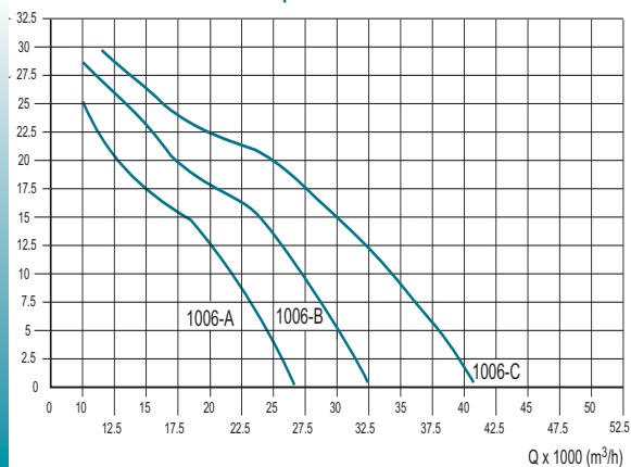
DUCT-M 1000 - 6 poles
