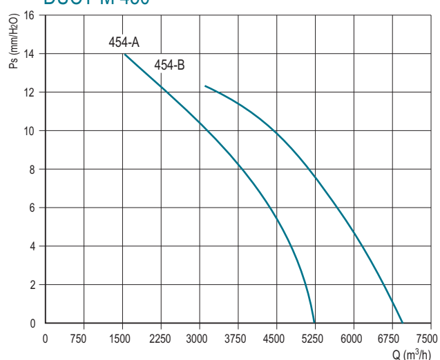
DUCT-M 450
