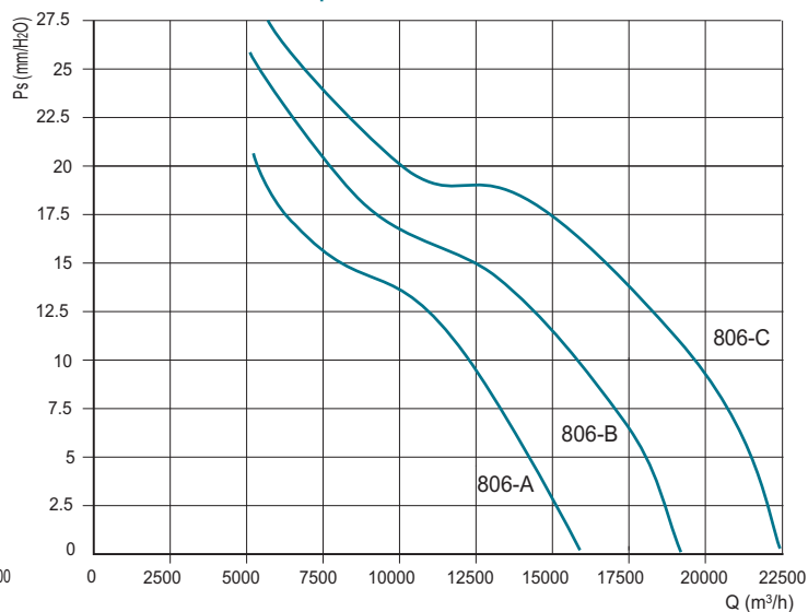
DUCT-M 800 - 6 poles
