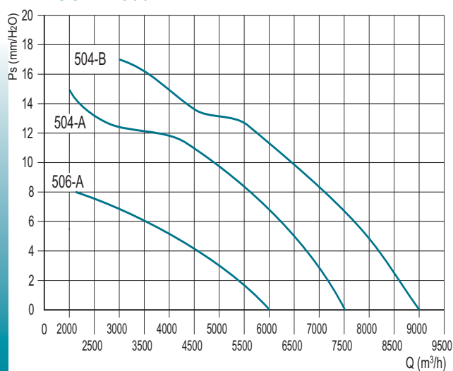
DUCT-M 500
